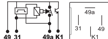
D9047 24V 4T 170W Mercedes Benz, Universal
