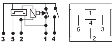
D0881 12V 5T 120W
